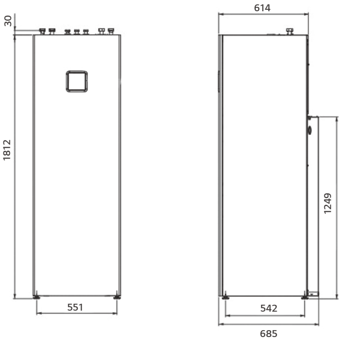
Combi Unit
